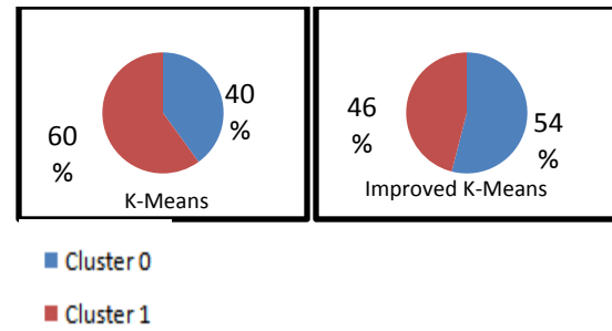
Figure 3: Seeds Dataset
